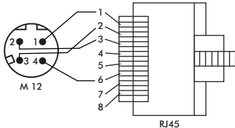
RJ45-Stecker
