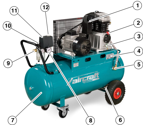
Abb. 8: AIRSTAR 503/100
