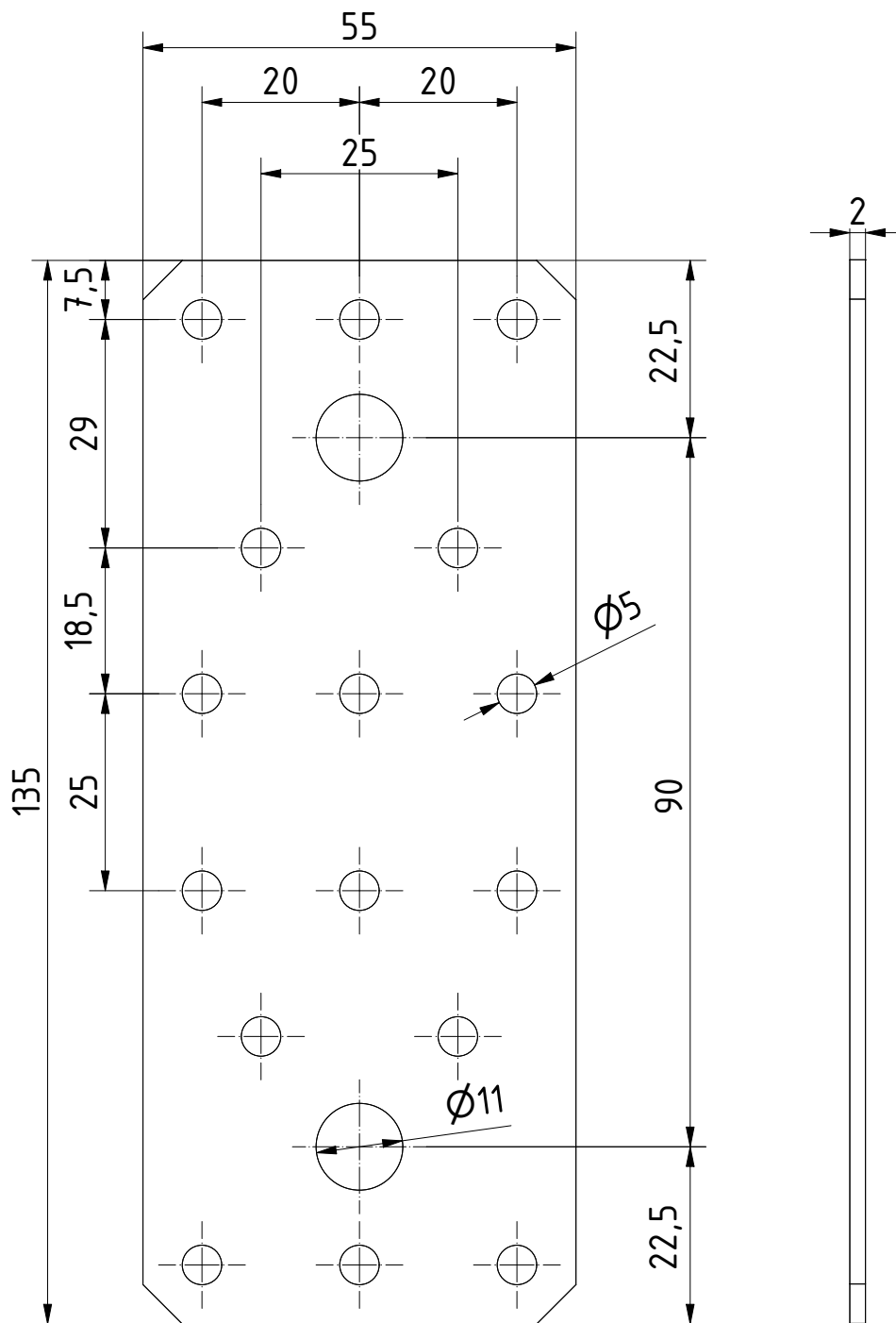
Front view
