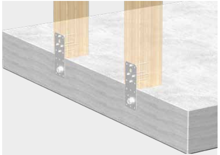
Simple assembly of two wooden elements on a concrete slab with the light flat connector.
