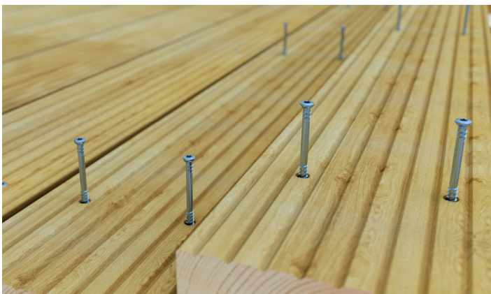
Sample application of the Terrasotec ornamental head in a decking board.
