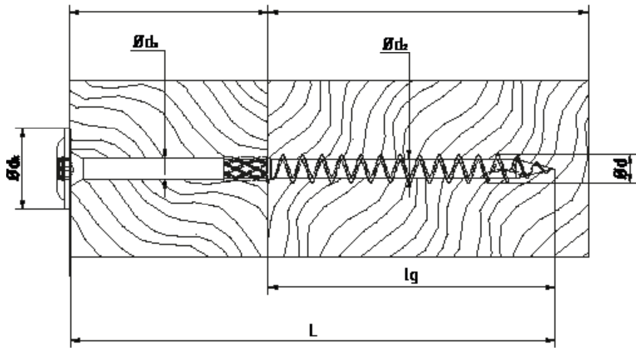
Side view
