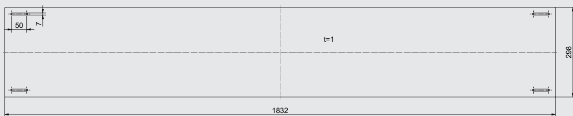
FLD-Windschutz
