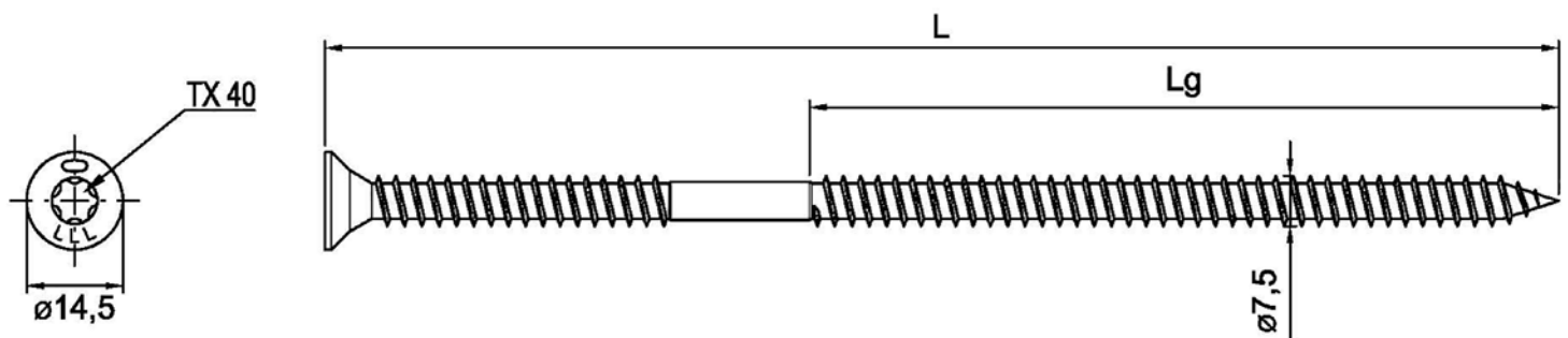
Blue-Power Systemschraube
